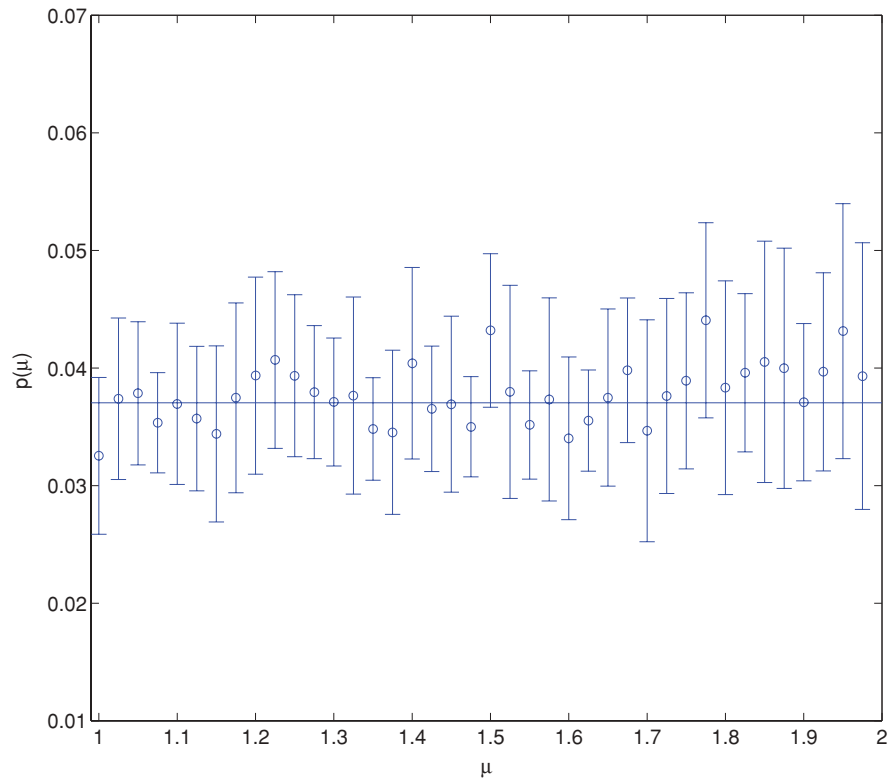
FIG. 11. (Color online) Plot of p(\mu) vs \mu for a system of volume 276, with error bars, for s = 3 . The line is p(\mu) = \frac{1}{3s^2} = \frac{1}{27} .
