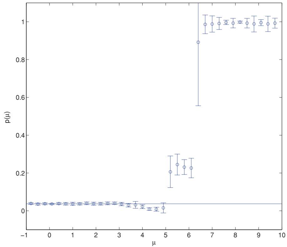
FIG. 10. (Color online) Plot of p(\mu) vs \mu for a system of volume 1151, with error bars, for s = 3 . The line is p(\mu) = \frac{1}{3s^2} = \frac{1}{27} .
