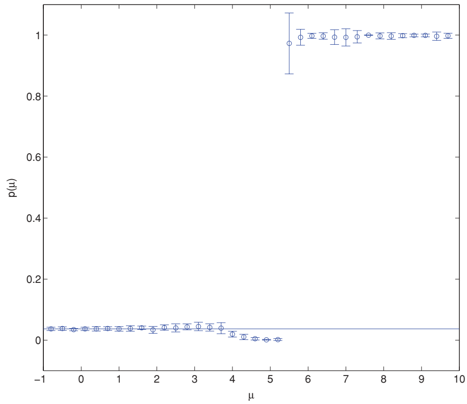
FIG. 9. (Color online) Plot of p(\mu) vs \mu for a system of volume 276, with error bars, for s = 3 . The line is p(\mu) = \frac{1}{3s^2} = \frac{1}{27} .
